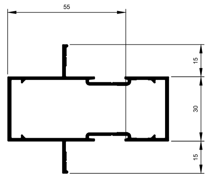
TSF007 Mullion 75mm 26 Ix: 23.198cm 4
