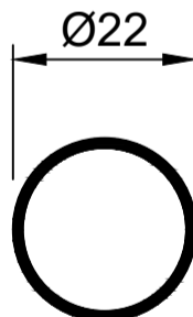
TRT002 Round Tube Dia 22.0mm x 1.2mm Ix: 0.431cm 4
