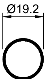
TRT001 Round Tube Dia 19.2 mm x 1.2mm Ix: 0.276cm 4
