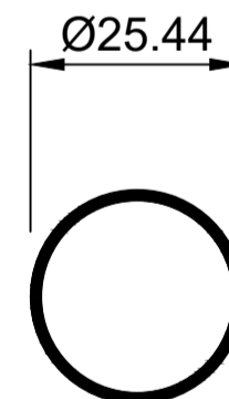
TRT003 Round Tube Dia 25.44 mm x 1.22mm Ix: 0.682cm 4
